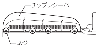
<MUH603SD>
